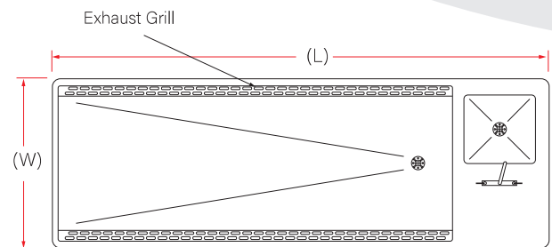
Top View Model : ATVA-2-S-D (with sink)
