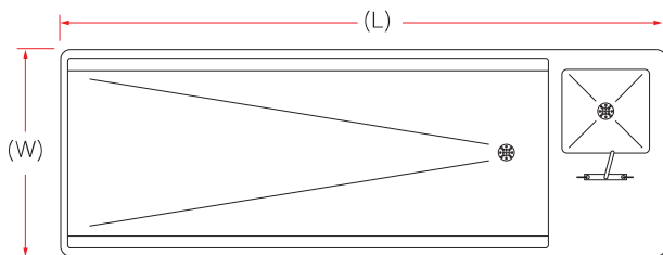
Top View Model : ATVA-2-S (with sink)
